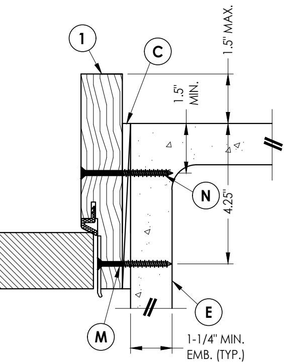
6 HORIZONTAL CROSS SECTION Shown Direct to Masonry Outswing only w/ 6-9/16" jamb
